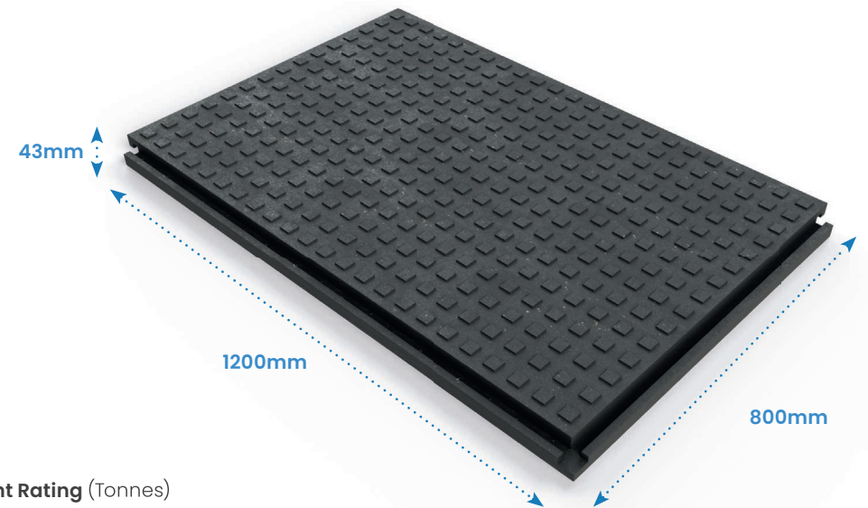
30mm Overlap Useable Surface 770 x 1170mm
